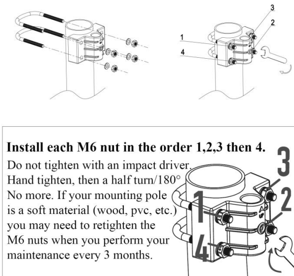
Figure 6: Sensor package mounting diagram 6-4
